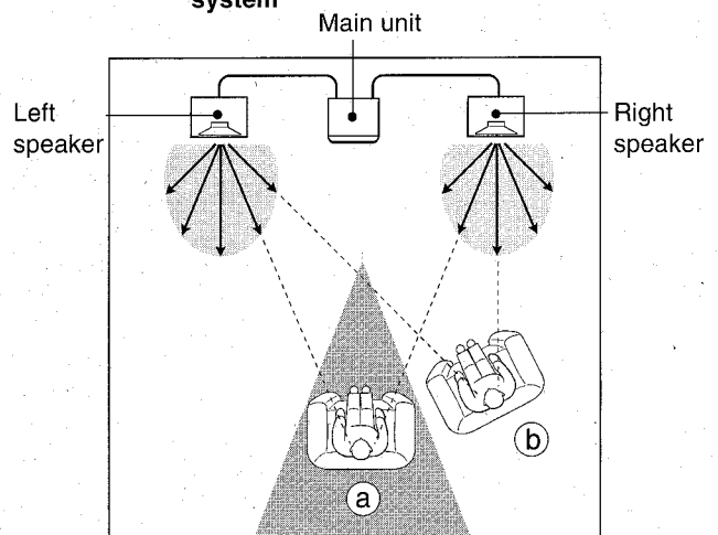
Figure 2 Stereo effect with a conventional speaker system
